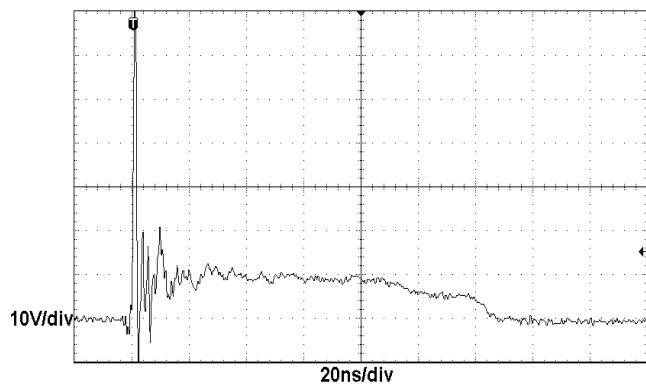
ESD clamping
