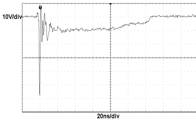
ESD clamping
