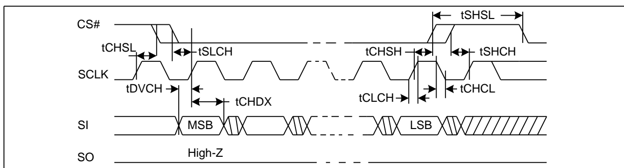
Figure 83. Input Timing
