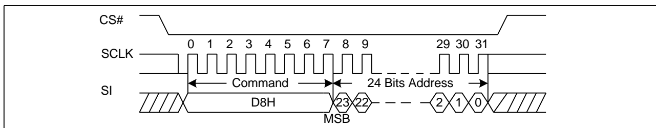
Figure 54. 64KB Block Erase Sequence Diagram (ADS=0)
