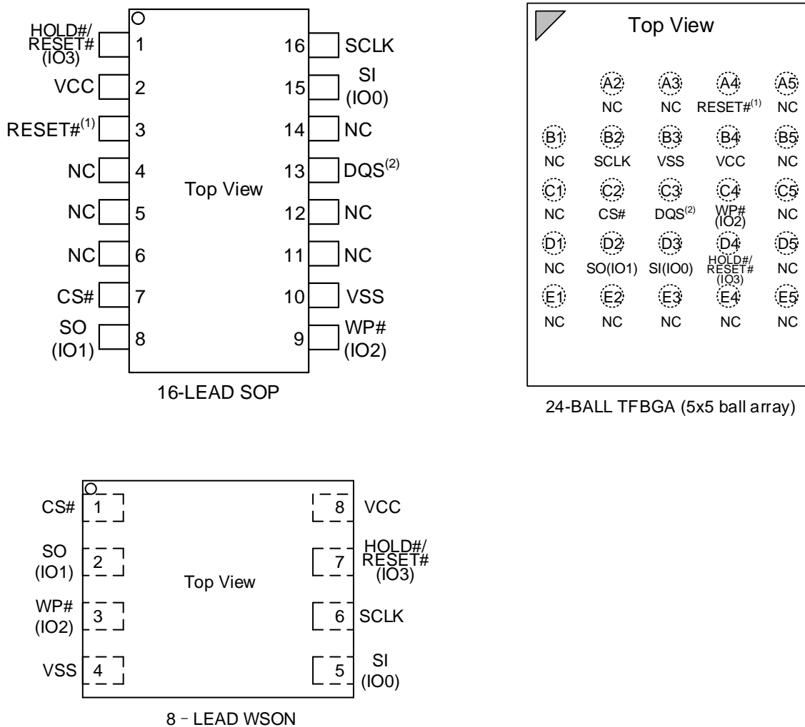
Figure 1 Connection Diagram
