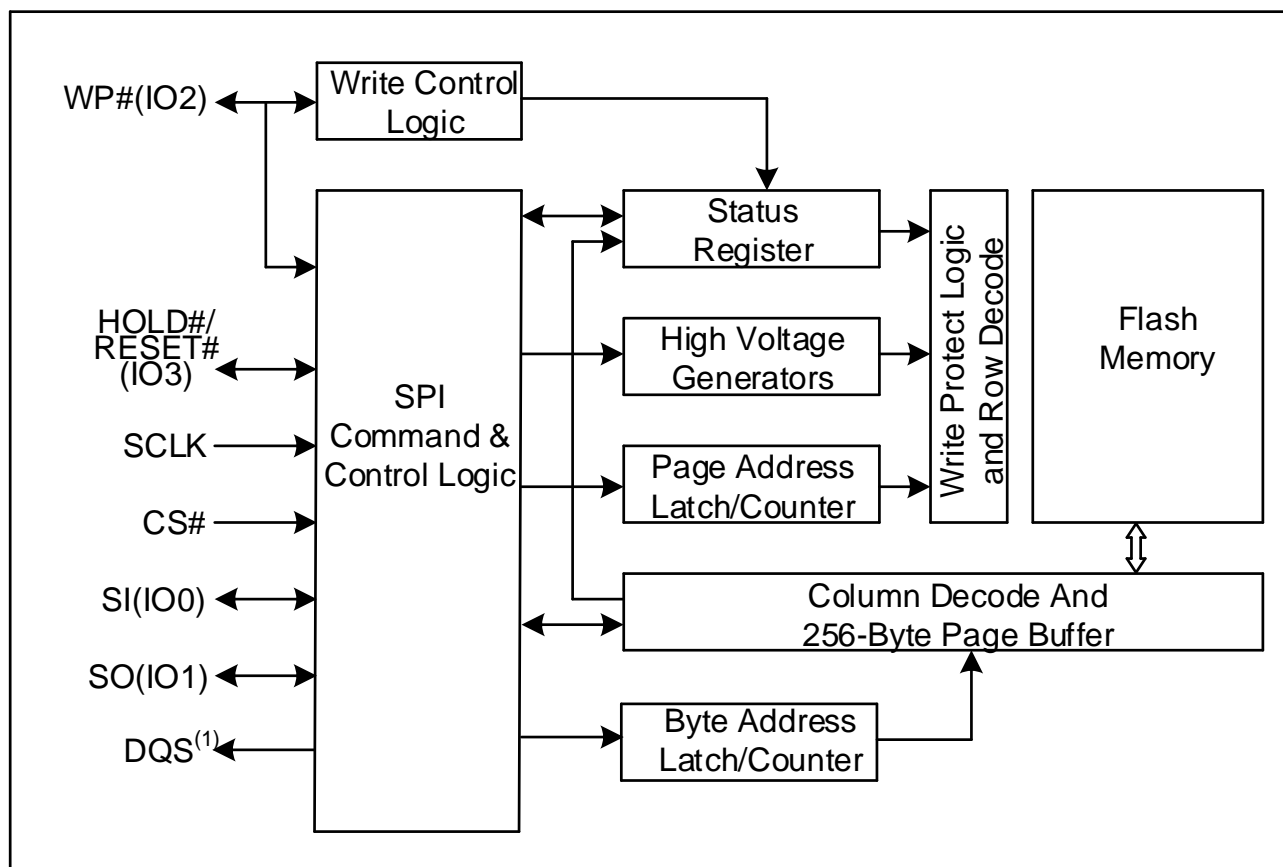
Figure 2 Block Diagram
