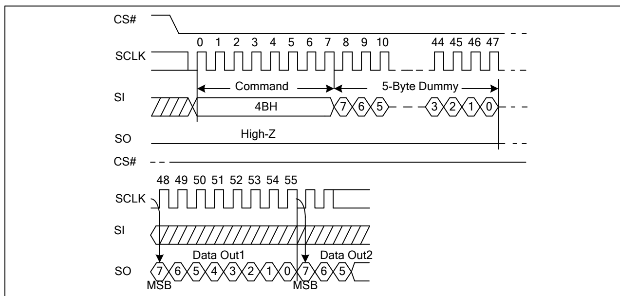
Figure 60. Read Unique ID Sequence Diagram (ADS=1)
