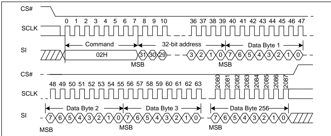
Figure 43. Page Program Sequence Diagram (ADS=1)
