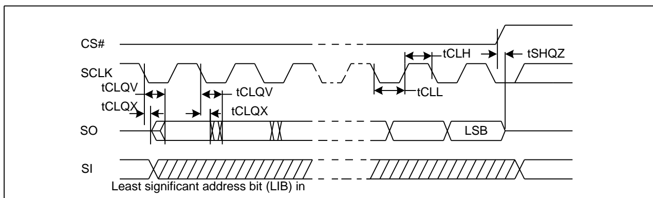
Figure 84. Output Timing
