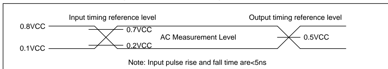
Figure 82. Input/Output Timing Reference Level
