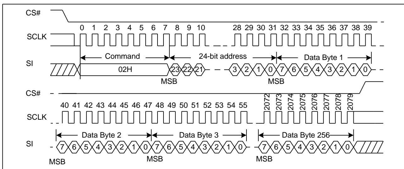
Figure 42. Page Program Sequence Diagram (ADS=0)
