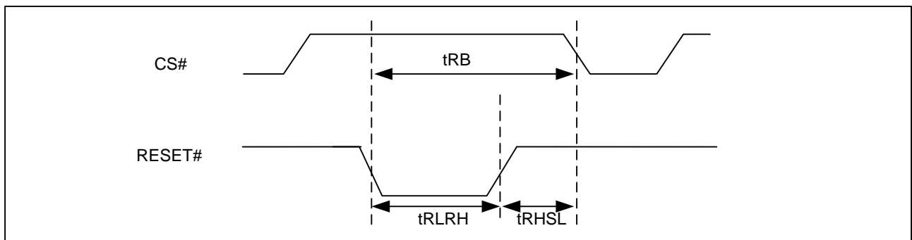
Figure 86. RESET Timing
